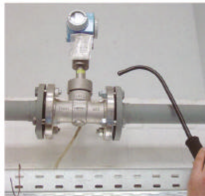
Picture below: a telescope bar offers a wide range for location of leaks (maximum length 3 m / 9.8 feet); large mobility by using a flexible probe
